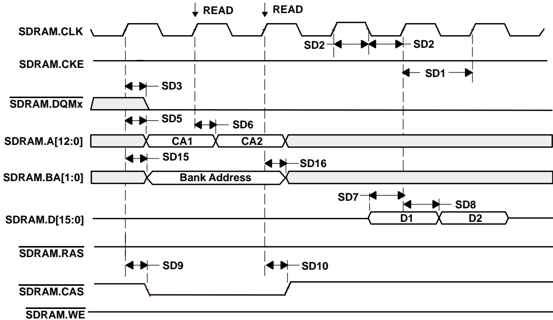
Figure 5–12. Two SDRAM RD (Read) Commands (Active Row)
