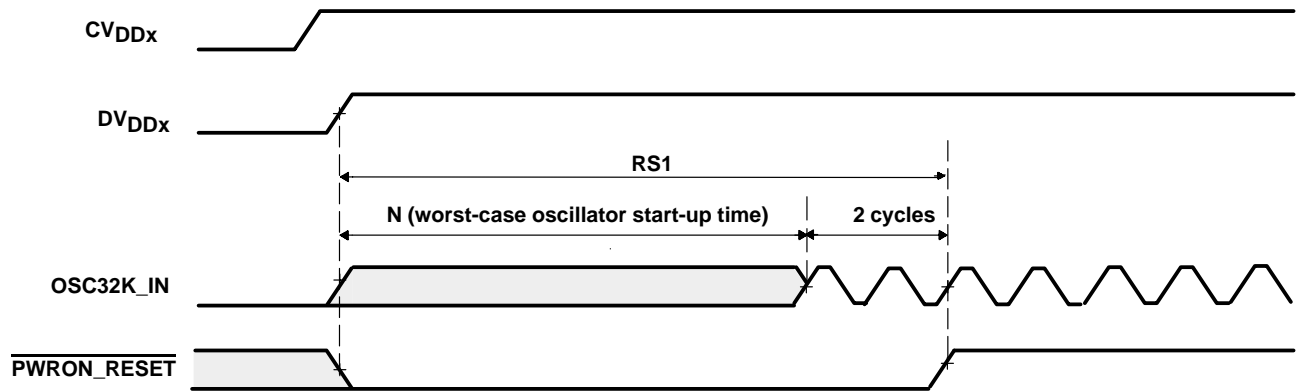
Figure 5–5. Device Reset Timings
