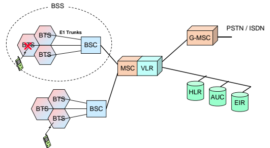
GSM Network Infrastructure
