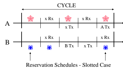
Reservation Schedules - Slotted Case
