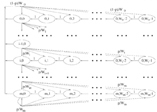
Wirt Fig. 3. Markov chain model for the backoff window size.
