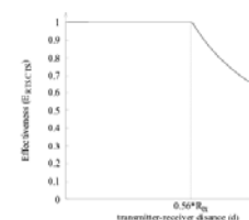
Fig. 2. Effectiveness of RTS/CTS handshake for TWO-RAY GROUND model and SNR threshold of 10.
