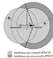
Fig. 1. Effectiveness of RTS/CTS handshake when d is larger than T_{SNR} + R_t and smaller than R_r .
