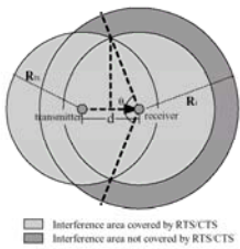
Fig. 1. Effectiveness of RTS/CTS handshake when d is large T_{SNR} \frac{1}{2} > R_{rx} and smaller than R_{tx} .
