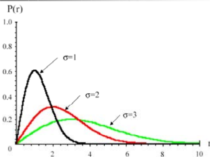
The pdf of the envelope variation
