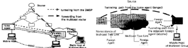
Fig. 4. Inefficient tunneling problem:
