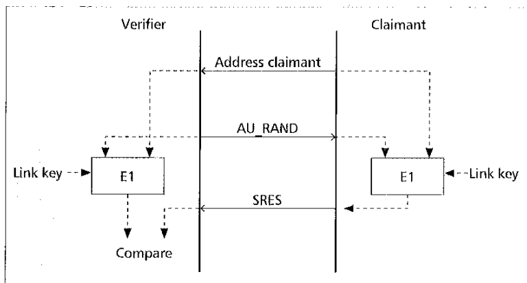
■ Figure 11. The Bluetooth authentication procedure.
